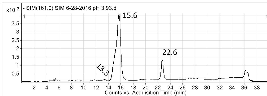
Figure 59. Extracted ion chromatogram of m/z 161 from a reaction performed at a pH of approximately 4.
