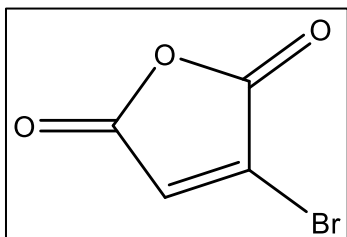
Figure 29. The structure of 3-bromo-2,5-furandione.
