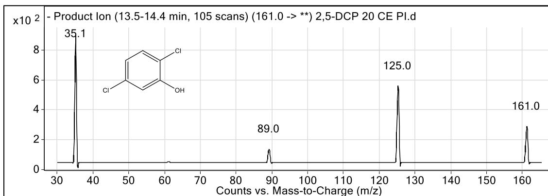
Figure 49. The structure of 2,5-dichlorophenol and its product ion spectrum of m/z 161 (the (M-H) - ion having a formula of ^{12}\text{C}_6\text{H}_3^{35}\text{Cl}_2\text{O} ).
