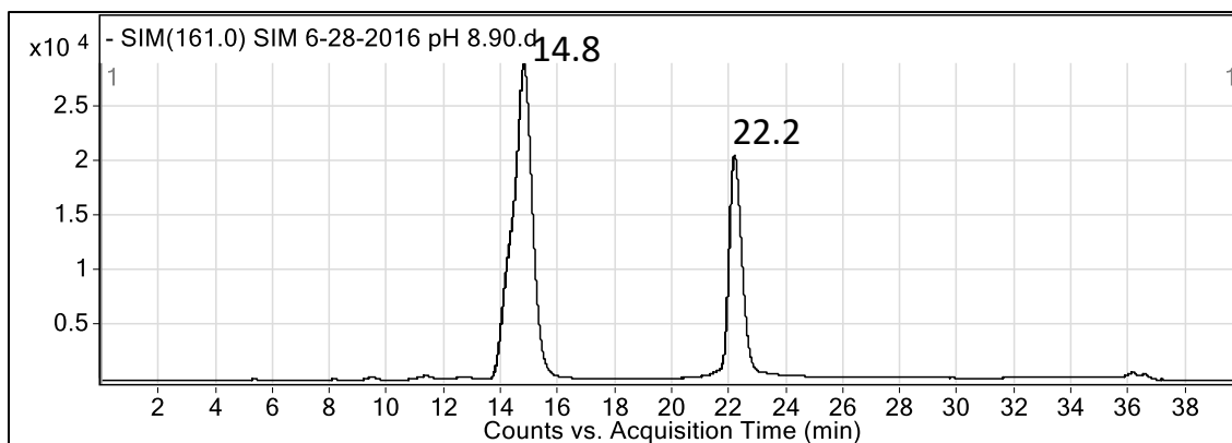
Figure 64. Extracted ion chromatogram of m/z 161 from a reaction performed at a pH of approximately 9.
