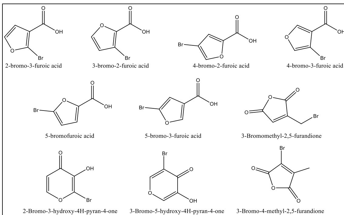
Figure 30. The proposed structures matching the formula C_5H_3BrO_3 .
