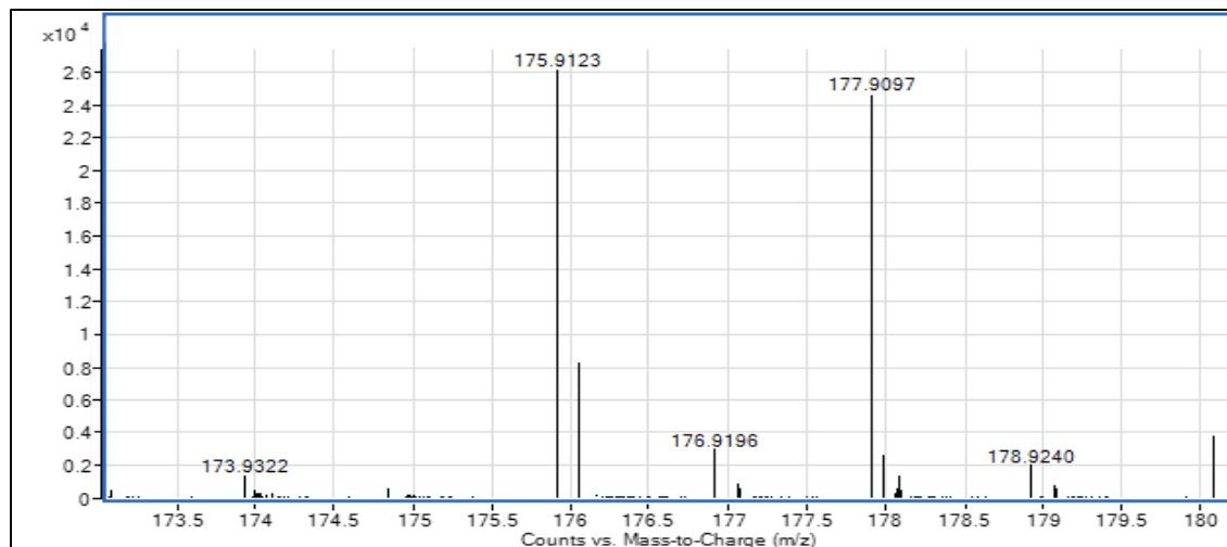
Figure 22. Mass spectrum of a monobrominated compound having monoisotopic masses at m/z 175.9123 and m/z 177.9097.
