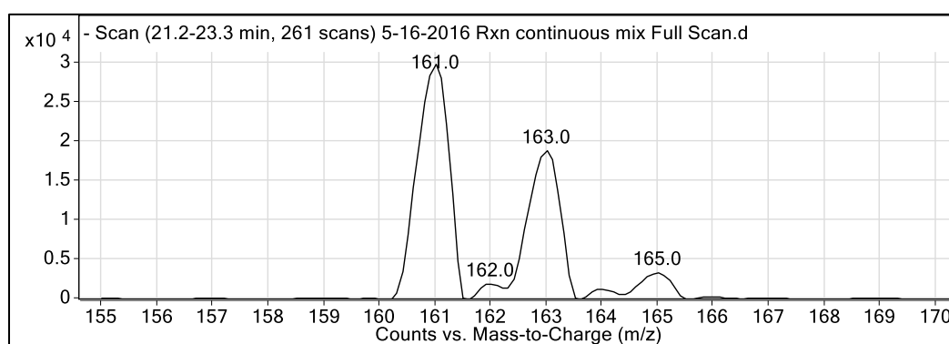
Figure 54. Full scan spectrum of the unknown peak centered at 22.5 minutes show a dichlorinated compound (isotope ratio of about 100:64:10).
