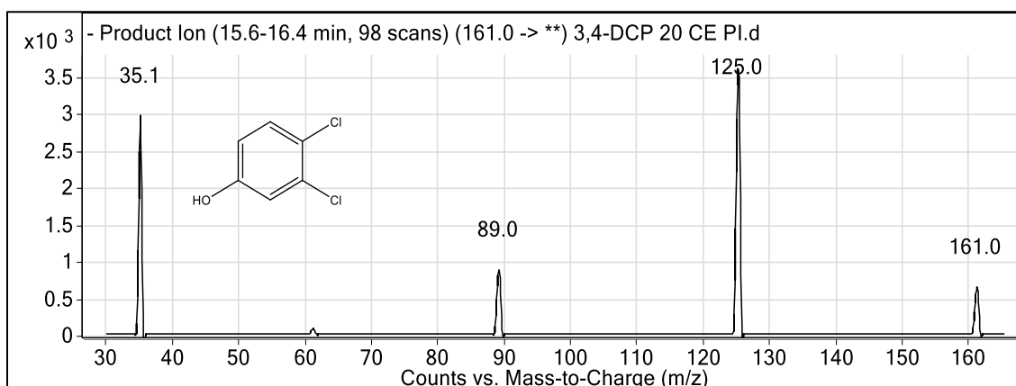
Figure 51. The structure of 3,4-dichlorophenol and its product ion spectrum of m/z 161 (the (M-H)^- ion having a formula of ^{12}C_6H_3^{35}Cl_2O ).
