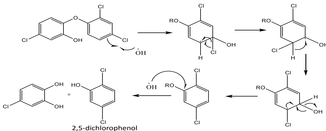
Scheme 12. The proposed mechanism of triclosan oxidation leading to the formation of 2,5-dichlorophenol.
