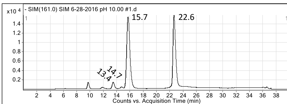
Figure 65. Extracted ion chromatogram of m/z 161 from a reaction performed at a pH of approximately 10.
