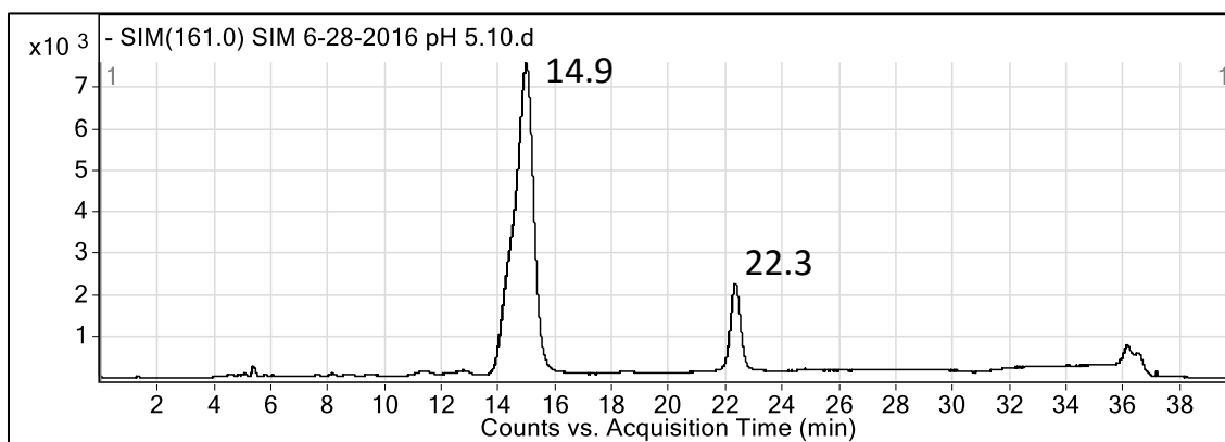
Figure 60. Extracted ion chromatogram of m/z 161 from a reaction performed at a pH of approximately 5.
