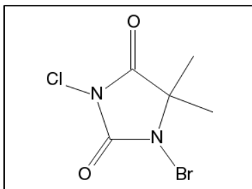
Figure 17. The structure of 3-bromo-1-chloro-5,5-dimethylhydantoin (BCDMH).
