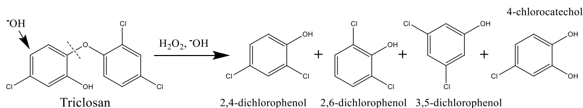
Scheme 10. Proposed formation of three isomeric dichlorophenols from the reaction of triclosan with hydrogen peroxide at a pH of approximately 10.
