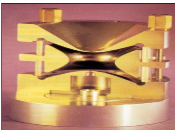
Figure 7. Example of an ion trap cut in half 122 .
