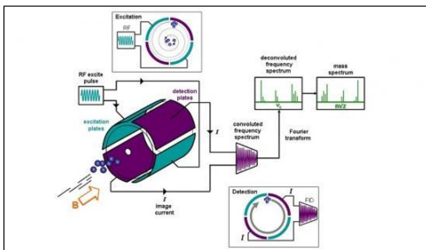
Figure 13. Schematic and operation of an FTICR-MS 128 .
