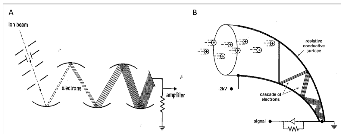
Figure 14. Diagrams of (A) a discrete dynode electron multiplier and (B) a continuous dynode electron multiplier 118 .
