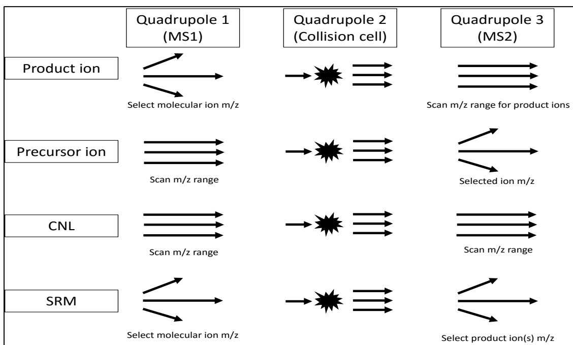
Figure 16. Schematic diagrams of MS/MS experiments.
