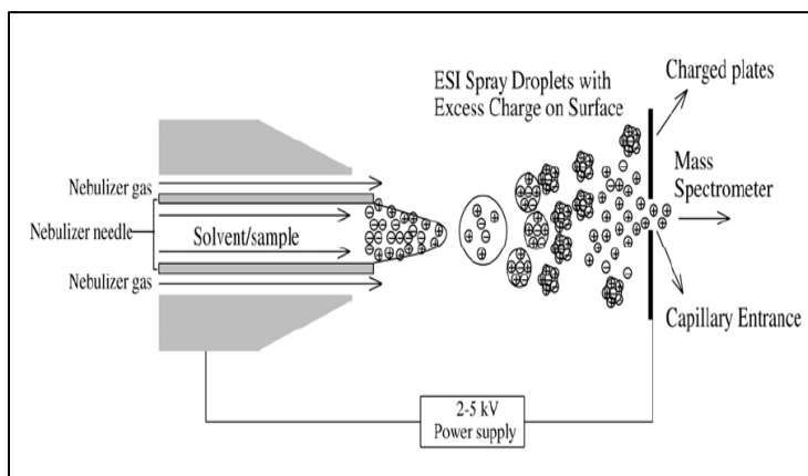
Figure 6. Schematic of electrospray ionization 119 .
