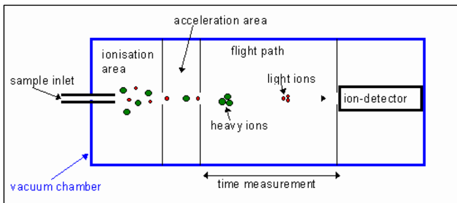
Figure 11. Diagram of the operation of a time-of-flight mass spectrometer 125 .
