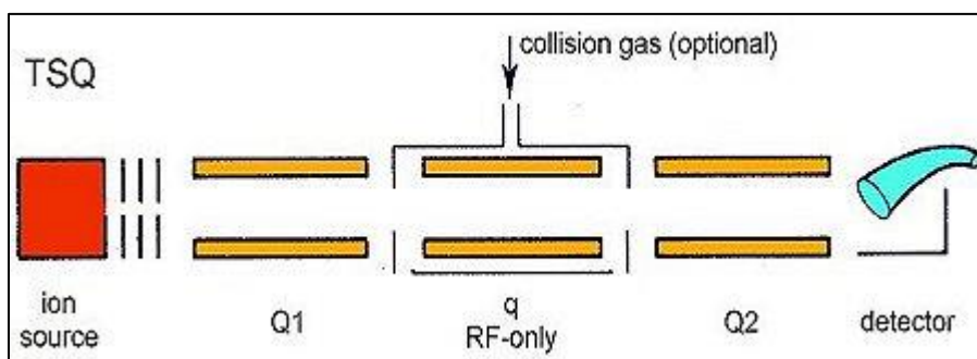
Figure 10. Configuration of a triple quadrupole mass spectrometer 123 .
