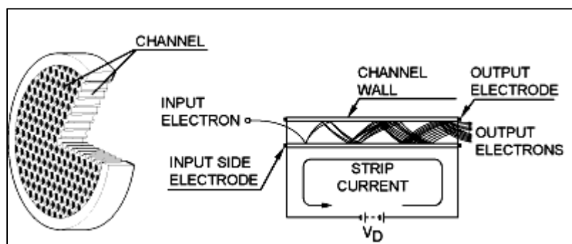
Figure 15. Schematic of a multichannel plate detector 129 .
