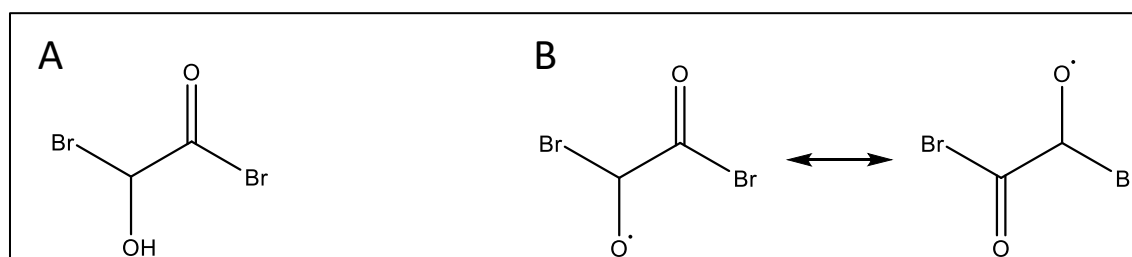
Figure 28. (A) The structure of 1,2-dibromo-1-hydroxy-2-oxo-ethane and (B) the resonance stabilized 1,2-dibromo-oxoethoxy radical.
