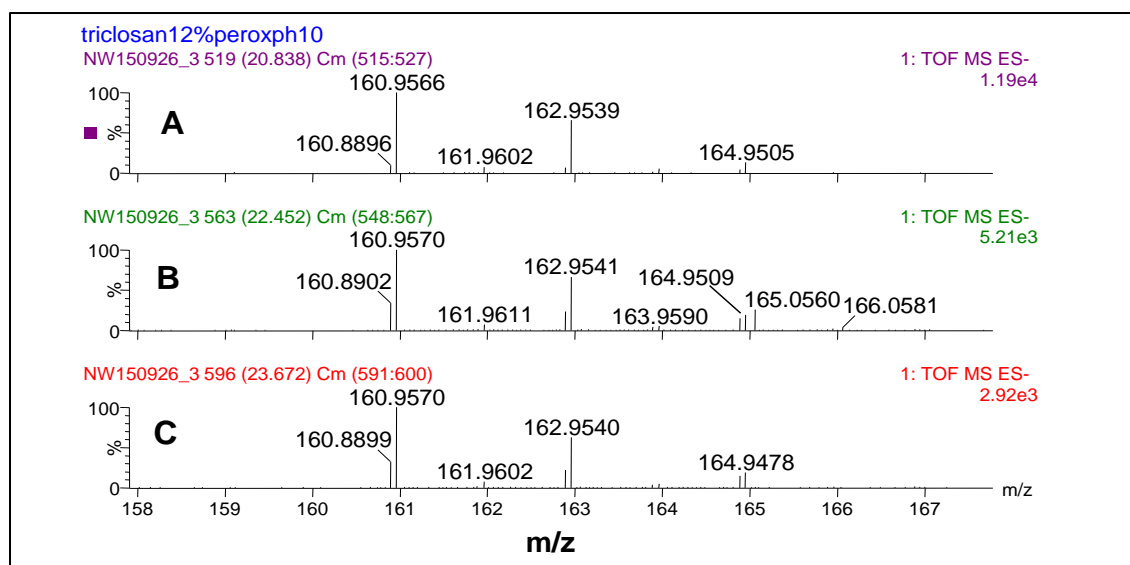
Figure 44. Negative ion LC-TOFMS spectra of the dichlorophenols eluting at (A) 21 minutes, (B) 22 minutes, and (C) 24 minutes.
