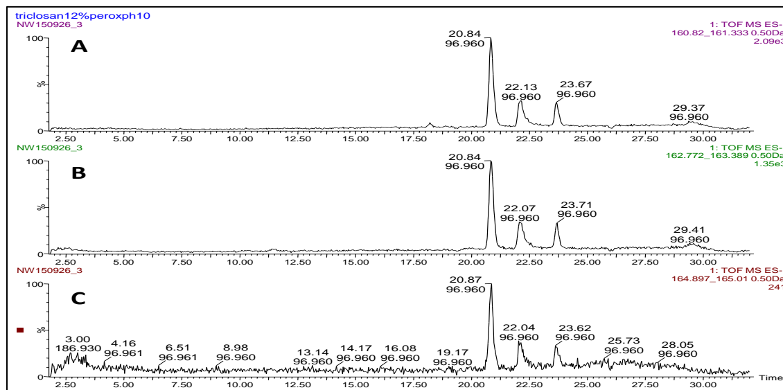
Figure 43. LC-TOFMS extracted ion chromatograms of the (A) m/z 160.9 ion, (B) m/z 162.9 ion, and (C) m/z 164.9 ion.
