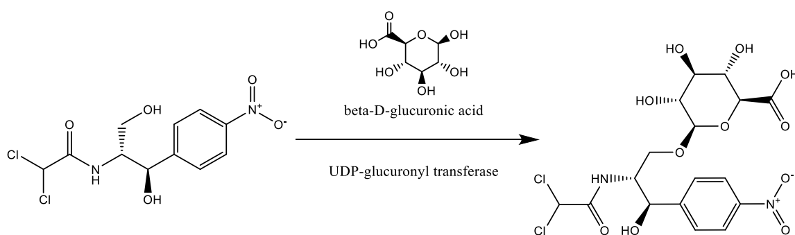
Scheme 2. Phase II glucuronidation of the antibiotic chloramphenicol.
