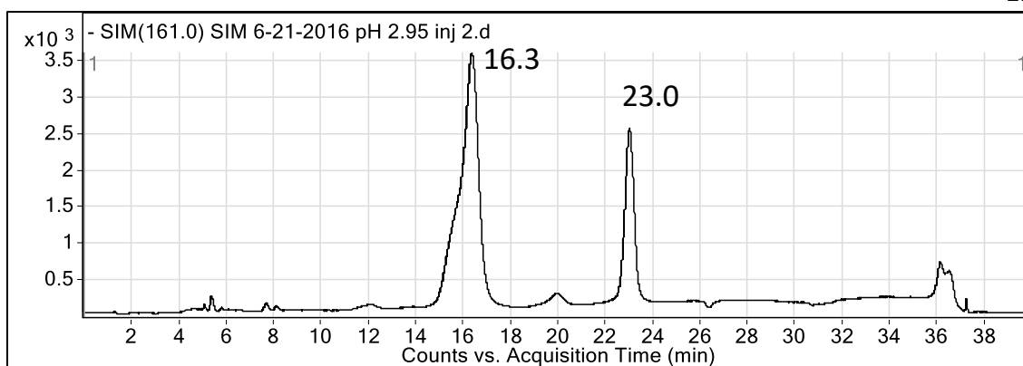
Figure 58. Extracted ion chromatogram of m/z 161 from a reaction performed at a pH of approximately 3.
