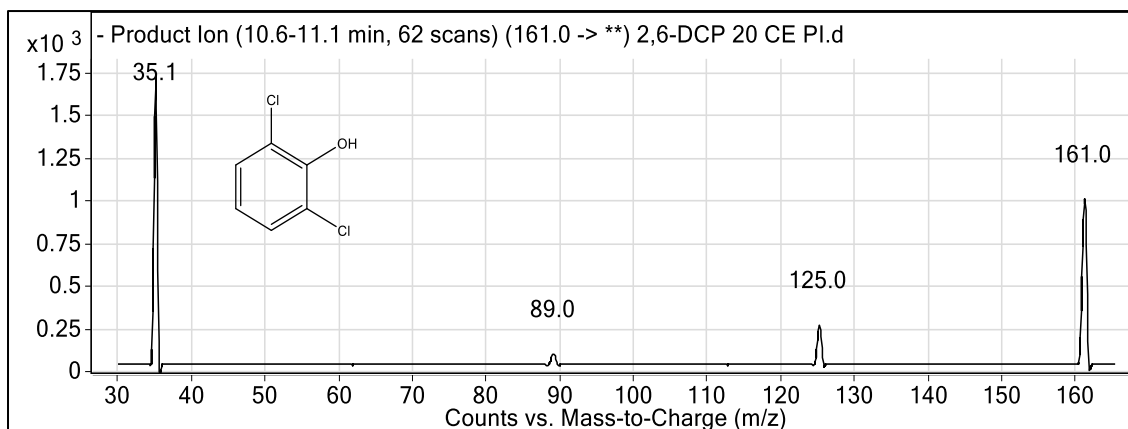
Figure 50. The structure of 2,6-dichlorophenol and its product ion spectrum of m/z 161 (the (M-H)^- ion having a formula of ^{12}C_6H_3^{35}Cl_2O ).
