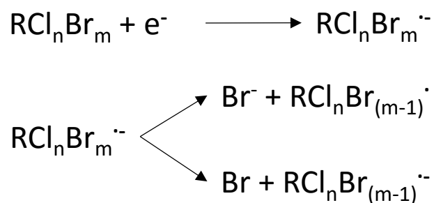
Scheme 7. The ionization and possible fragmentation of a halogenated compound in TD-NCI.
