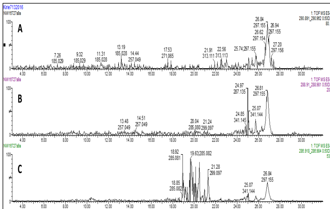
Figure 41. LC-TOFMS extracted ion chromatograms of the (A) m/z 290.9 ion, (B) m/z 288.9 ion, and (C) m/z 286.9 ion of the ^{35}\text{Cl} and ^{37}\text{Cl} isotopologues of triclosan.
