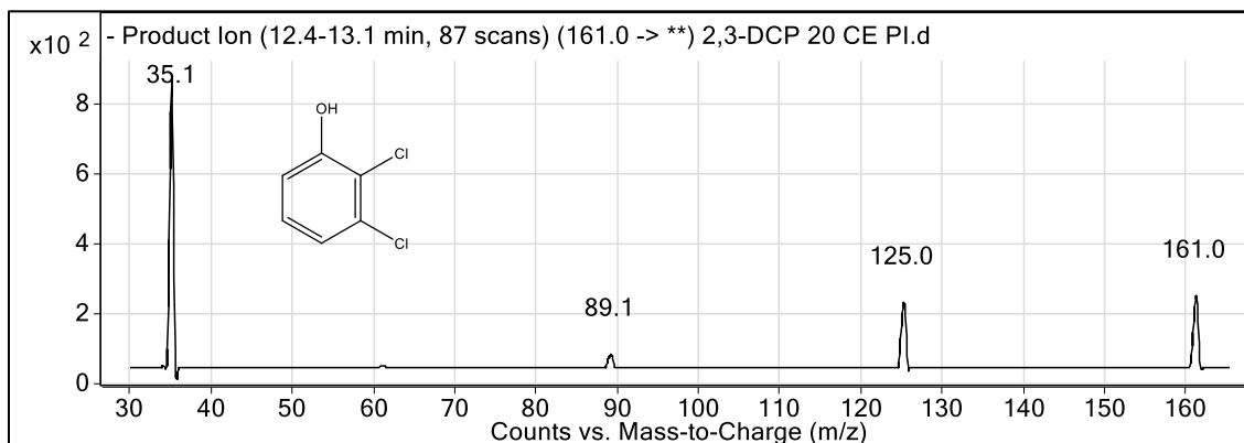
Figure 47. The structure of 2,3-dichlorophenol and its product ion spectrum of m/z 161 (the (M-H) - ion having a formula of ^{12}\text{C}_6\text{H}_3^{35}\text{Cl}_2\text{O} ).
