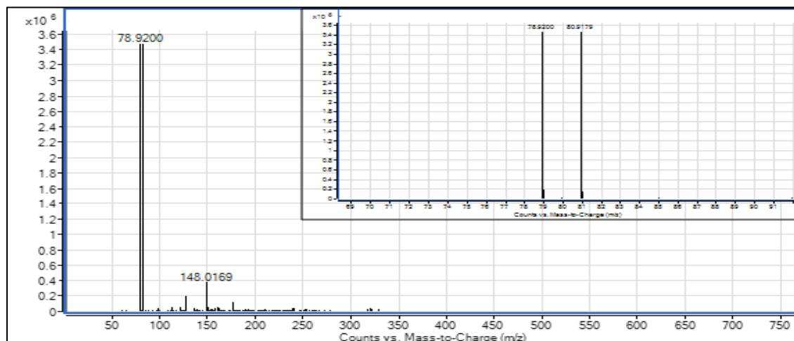
Figure 19. TD-NCI-TOF-MS full scan mass spectrum averaged over minutes 4-13 (inset showing exact isotope masses).
