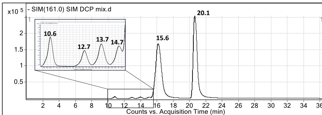
Figure 57. Extracted ion chromatogram of m/z 161 from a mixture of the six dichlorophenol standards each at a concentration of 167 \mu\text{g/mL} .
