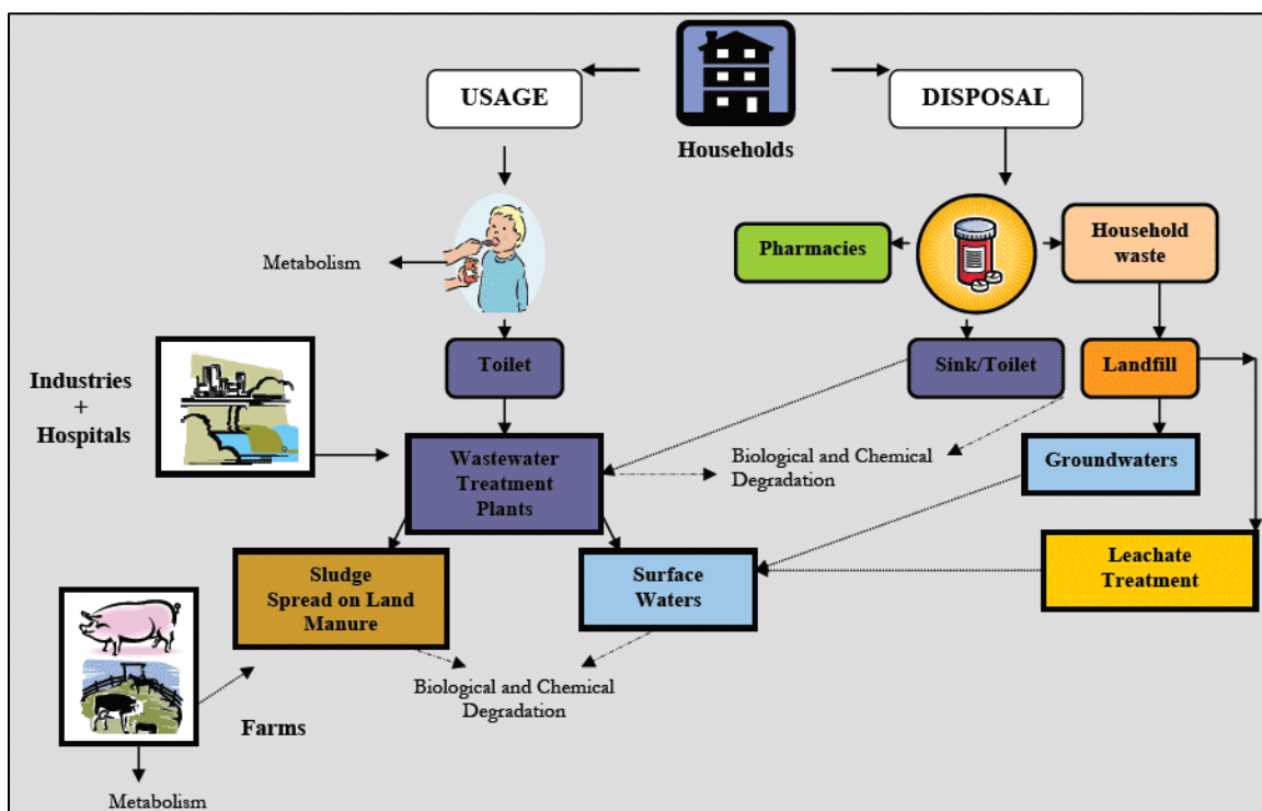
Figure 2. Sources of emerging contaminants 216 .
