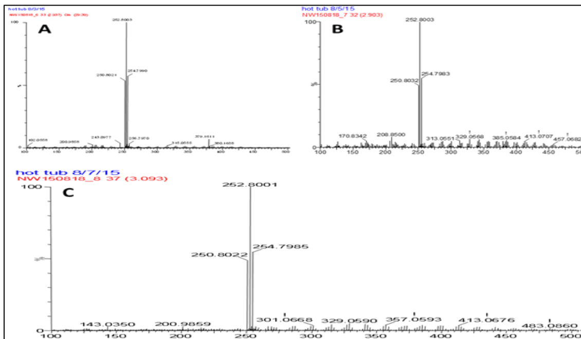
Figure 35. LC-TOF-MS full scan of a dibrominated ion at m/z 250.8/252.8/254.8 from the sampling of a hot tub on (A) Monday, (B) Wednesday, and (C) Friday in the same week.
