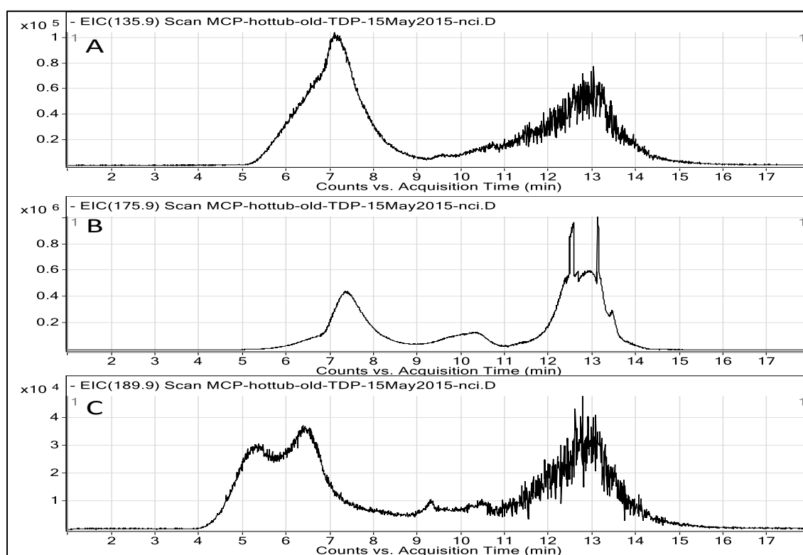
Figure 24. TD-NCI-TOF-MS extracted ion chromatograms for the (A) m/z 135.9 ion, (B) m/z 175.9 ion, and (C) m/z 189.9 ion.
