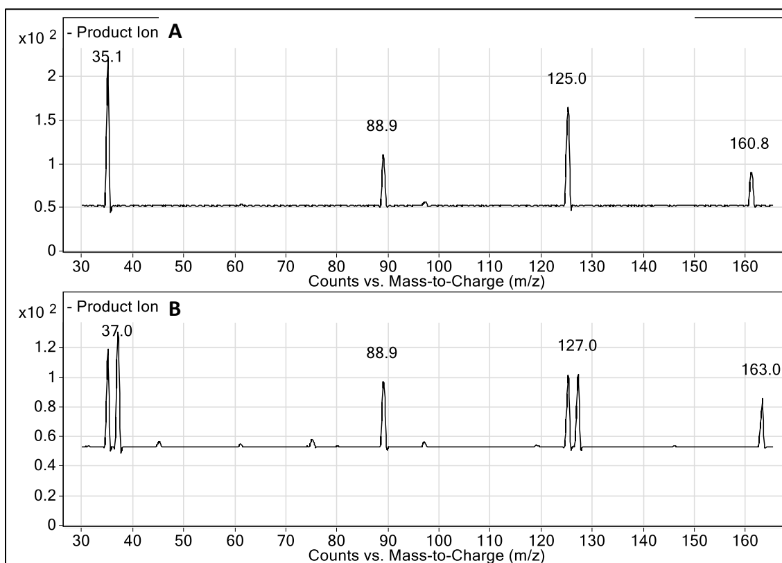
Figure 46. Product ion spectra of the (A) m/z 161 and (B) m/z 163 molecular ions for the unknown eluting at 15.8 minutes.
