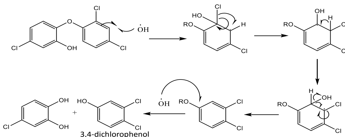
Scheme 11. The proposed mechanism of triclosan oxidation leading to the formation of 3,4-dichlorophenol.
