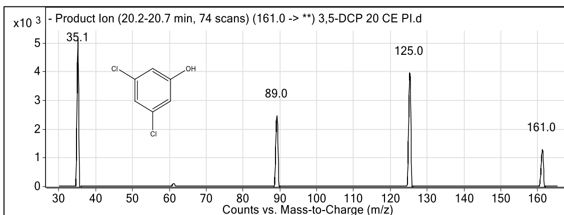
Figure 52. The structure of 3,5-dichlorophenol and its product ion spectrum of m/z 161 (the (M-H)^- ion having a formula of ^{12}C_6H_3^{35}Cl_2O ).
