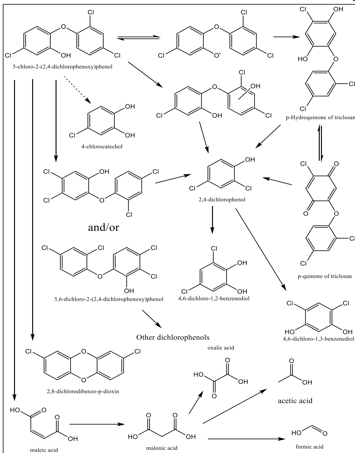
Scheme 3. Proposed pathways for the degradation of triclosan in the environment and advanced oxidation water treatment processes (modified and adapted from 113, 114, 116).
