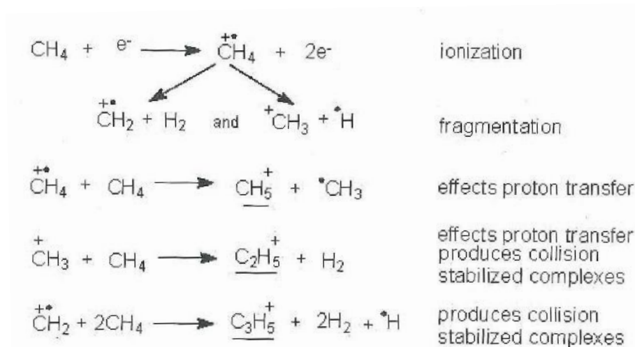
Scheme 4. Reactions for the ionization of the reagent gas in positive chemical ionization 118 .
