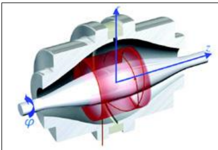
Figure 12. Cutaway of an orbitrap mass analyzer 127 .
