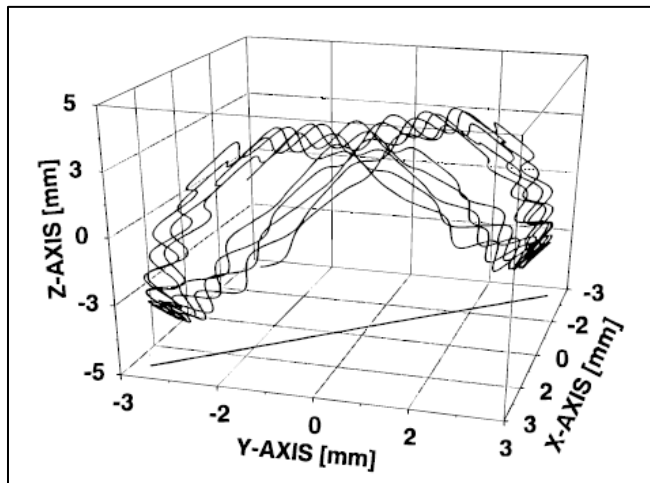
Figure 8. Modeled trajectory of an ion having a mass-to-charge ratio of 105 trapped in a 3-dimensional ion trap mass analyzer 122 .
