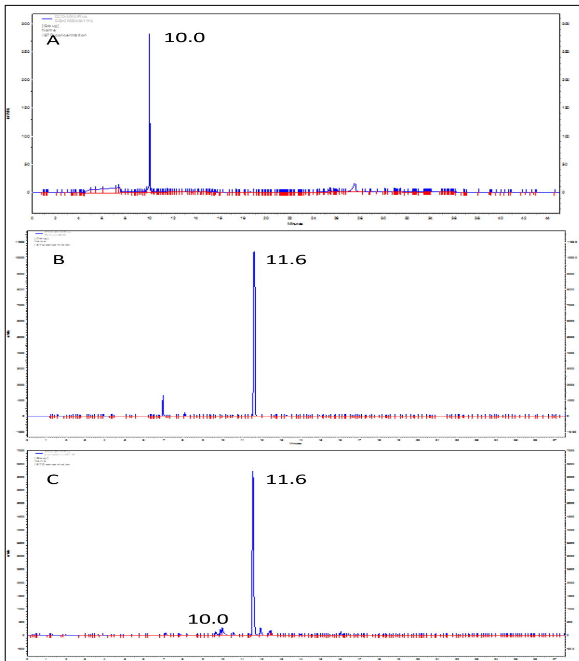
Figure 18. GC-ECD chromatograms of (A) dibromochloromethane, (B) bromoform, and (C) an extract of hot tub water.
