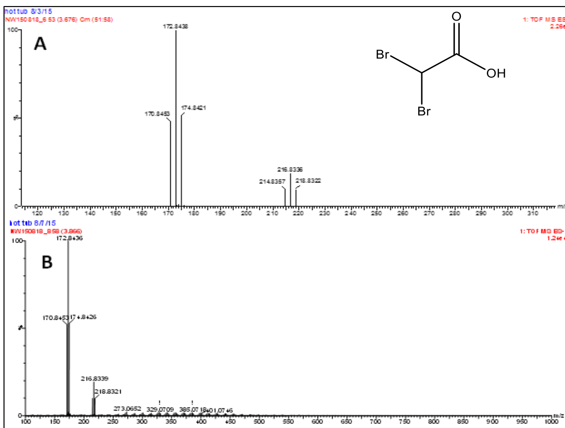
Figure 31. LC-TOF-MS full scan of dibrominated ions at m/z 170.8/172.8/174.8 and m/z 214.8/216.8/218.8 from the hot tub sample collected on (A) Monday (with the structure of dibromoacetic acid inset) and (B) Friday.
