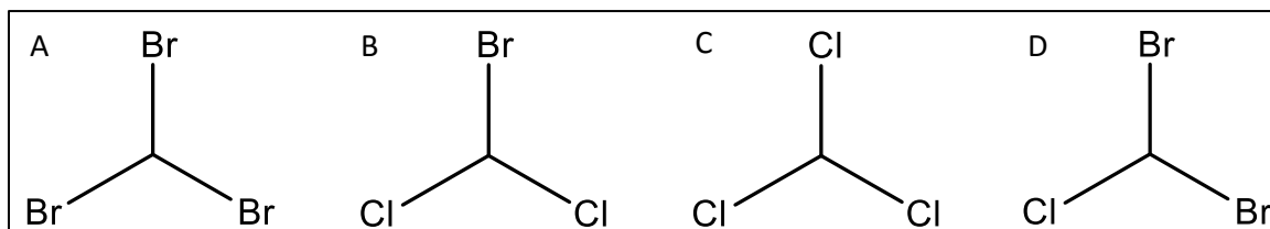
Figure 3. Structures of the four EPA regulated THMs: (A) bromoform, (B) bromodichloromethane, (C) chloroform, and (D) dibromochloromethane.
