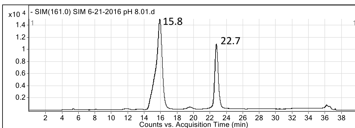
Figure 63. Extracted ion chromatogram of m/z 161 from a reaction performed at a pH of approximately 8.
