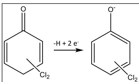
Figure 56. A proposed mechanism for ionization of the hypothesized semi-quinone structure (reactant) using ESI.
