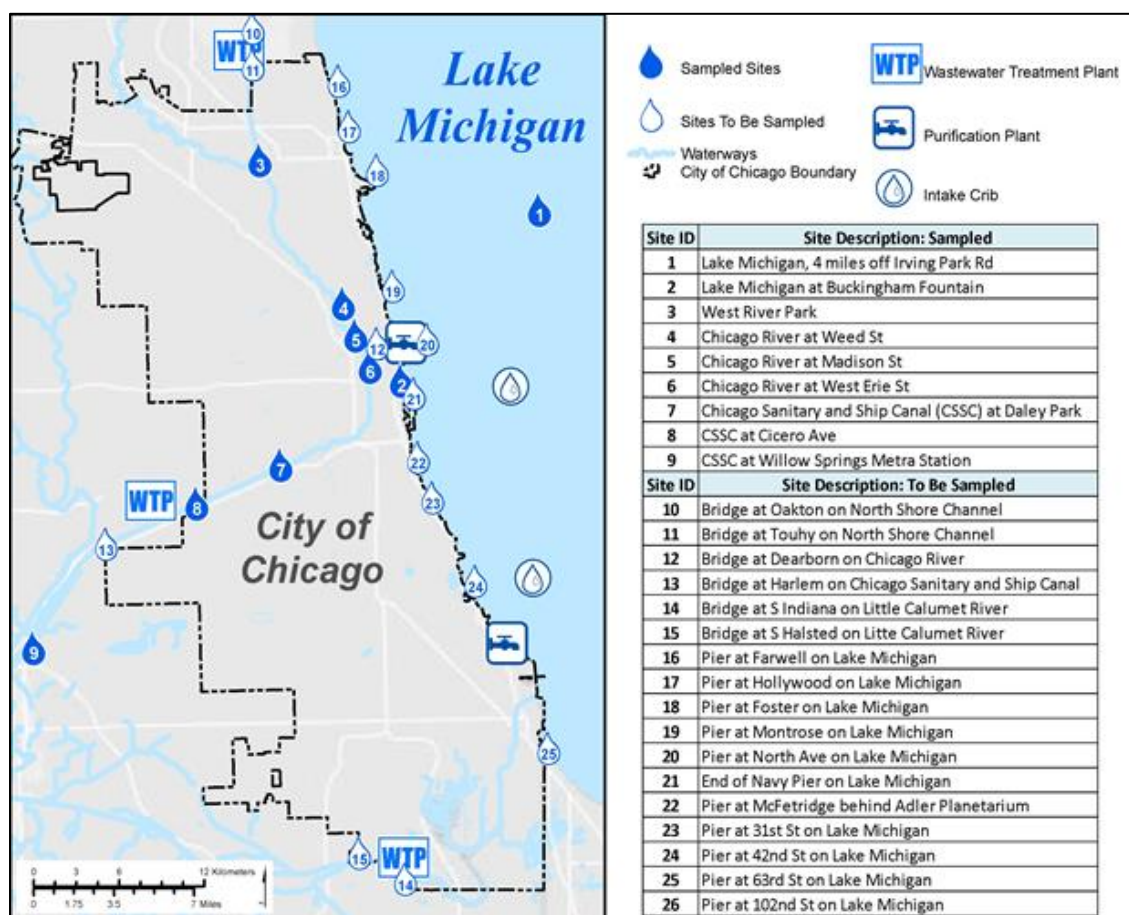
Figure 1. Map of Chicago area Lake Michigan shoreline and waterways with sampling points indicated by drops (CSSC = Chicago Sanitary and Ship Canal).
