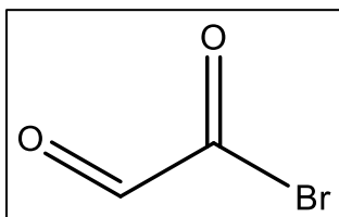
Figure 27. The structure of 2-oxoacetyl bromide.
