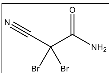
Figure 34. The structure of 2,2-dibromo-2-cyanoacetamide.
