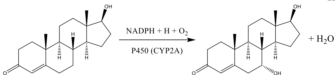
Scheme 1. Phase I biotransformation of testosterone by hydroxylation.
