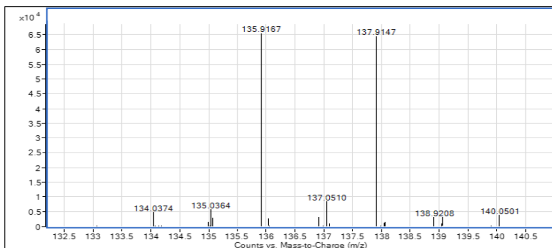
Figure 21. Mass spectrum of a monobrominated compound having monoisotopic masses at m/z 135.9167 and m/z 137.9147.
