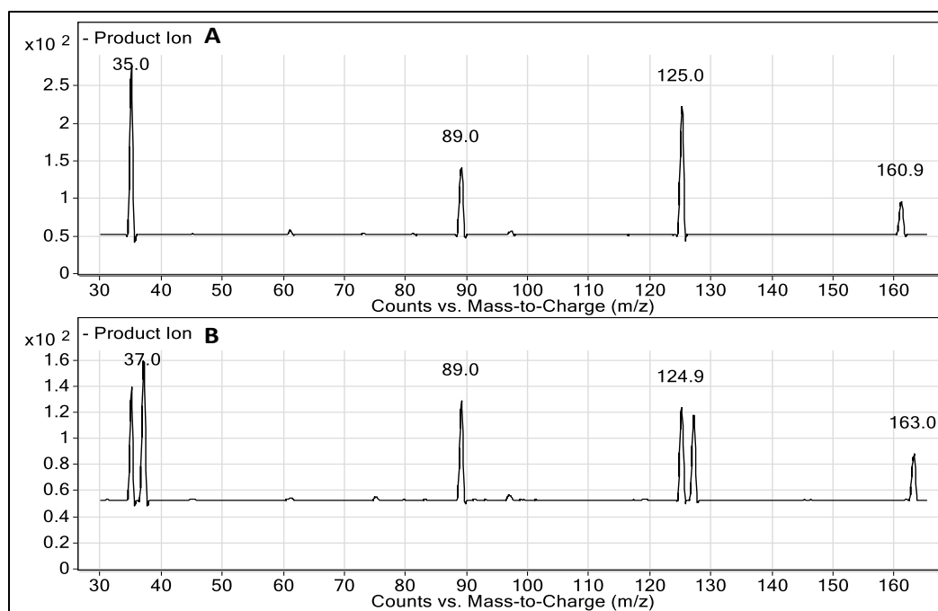
Figure 55. Product ion spectra of the late eluting peak for (A) m/z 161 and (B) m/z 163.
