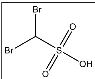
Figure 36. The structure of 1,1-dibromo-methanesulfonic acid.
