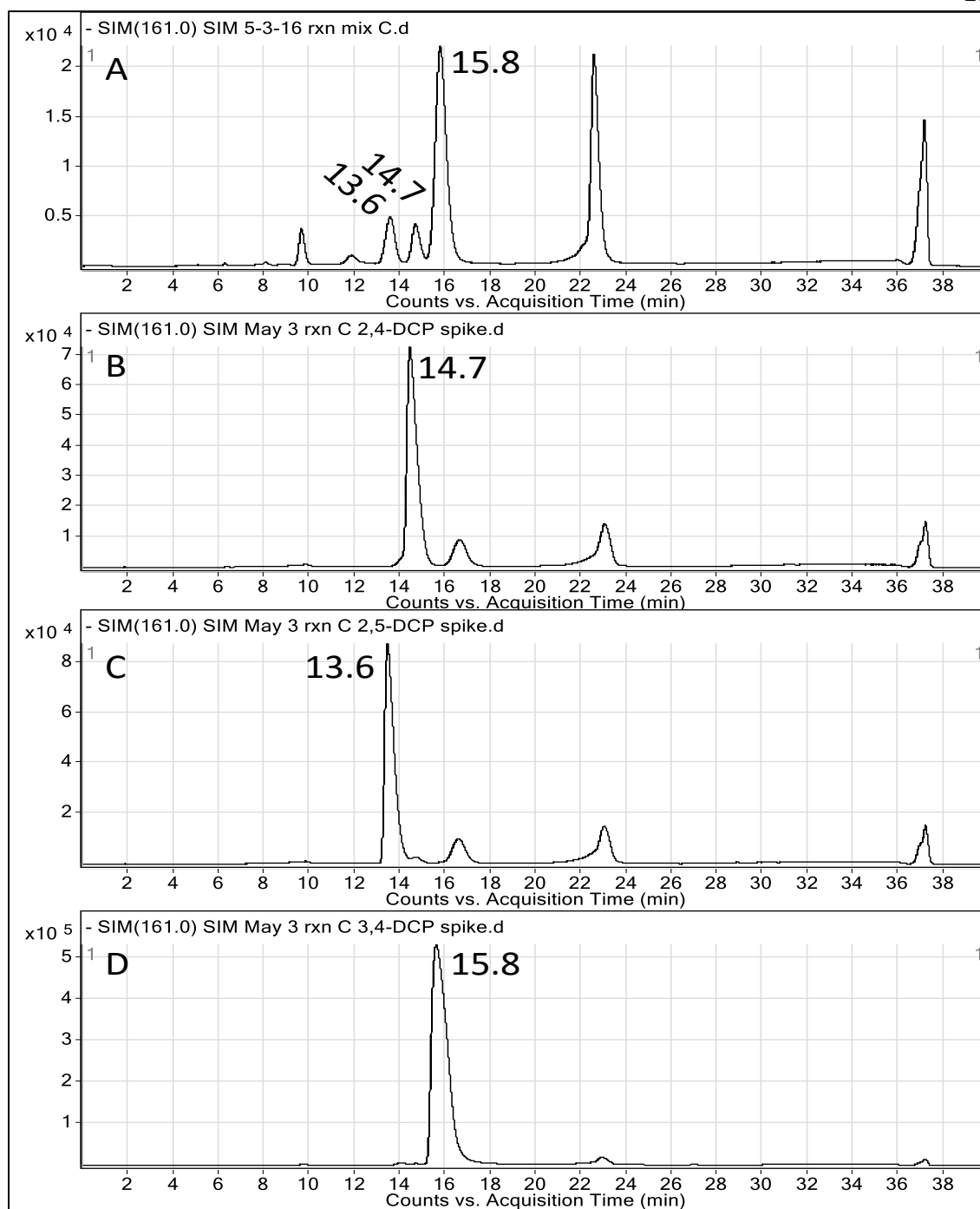
Figure 53. Extracted ion chromatograms of m/z 161 from a pH 10 reaction (A) not spiked, and spiked with (B) 2,4-dichlorophenol, (C) 2,5-dichlorophenol, and (D) 3,4-dichlorophenol.
