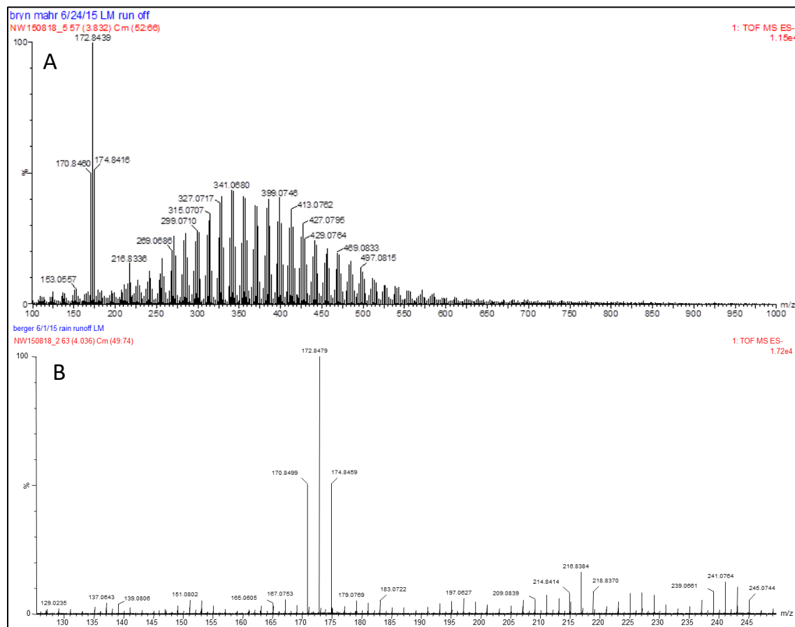
Figure 32. LC-TOF-MS full scan mass spectra of samples from Lake Michigan at (A) W. Bryn Mawr Ave. and (B) Berger Park indicating the presence of dibromoacetic acid.
