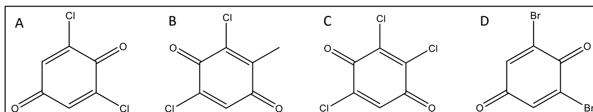
Figure 4. Structures of (A) 2,6-dichloro-1,4-benzoquinone, (B) 2,6-dichloro-3-methyl-1,4-benzoquinone, (C) 2,3,6-trichloro-1,4-benzoquinone, and (D) 2,6-dibromo-1,4-benzoquinone.
