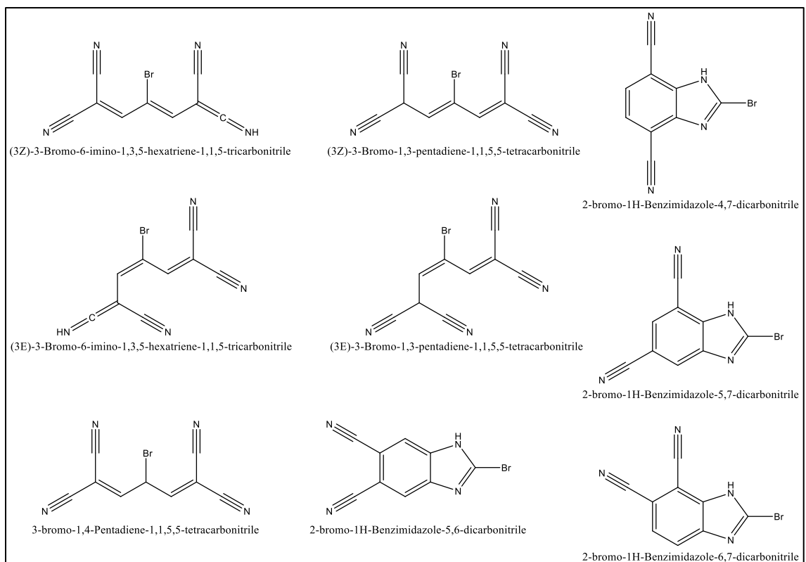
Figure 38. The nine structural matches for the formula C_9H_3BrN_4 that fit within 0.4 ppm mass accuracy.
