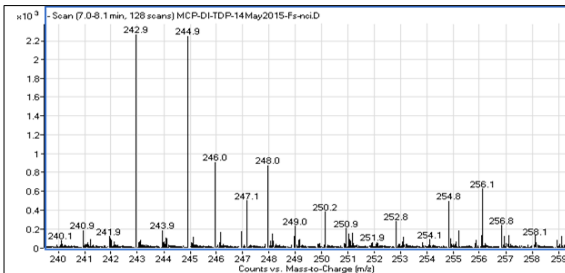
Figure 37. NCI-TOF mass spectrum of two monobrominated ions at ( m/z 242.9/244.9 and m/z 246.0/248.0) from the 24 hour extract of BCDMH in ultrapure water.
