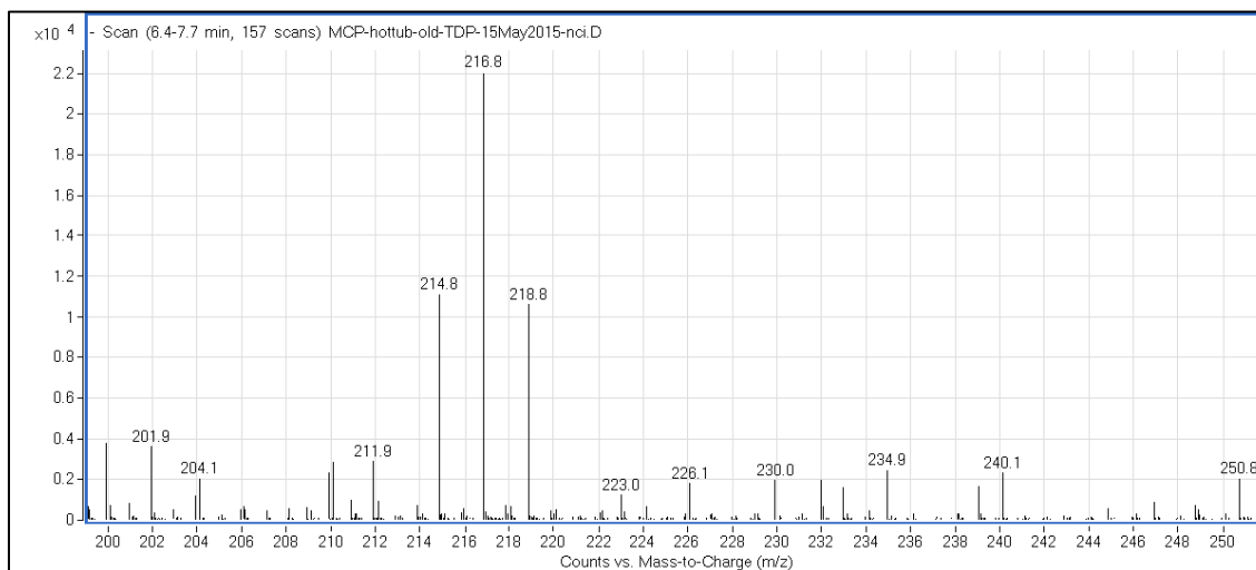
Figure 25. Mass spectrum of a dibrominated compound having monoisotopic masses at m/z 214.8337, m/z 216.8317 and m/z 218.8296.
