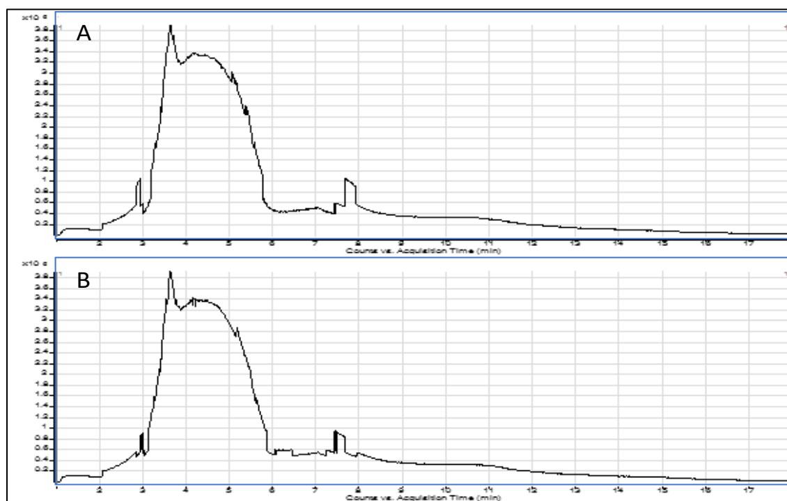
Figure 20. TD-NCI-TOF-MS extracted ion chromatogram for (A) m/z 79 and (B) m/z 81.
