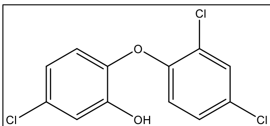
Figure 39. The structure of triclosan.
