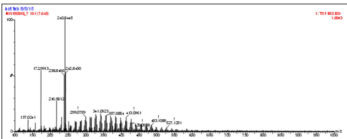
Figure 33. LC-TOF-MS full scan of a dibrominated ion at m/z 238.8/240.8/242.8.
