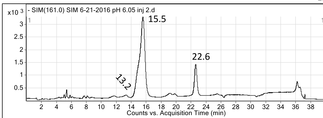
Figure 61. Extracted ion chromatogram of m/z 161 from a reaction performed at a pH of approximately 6.
