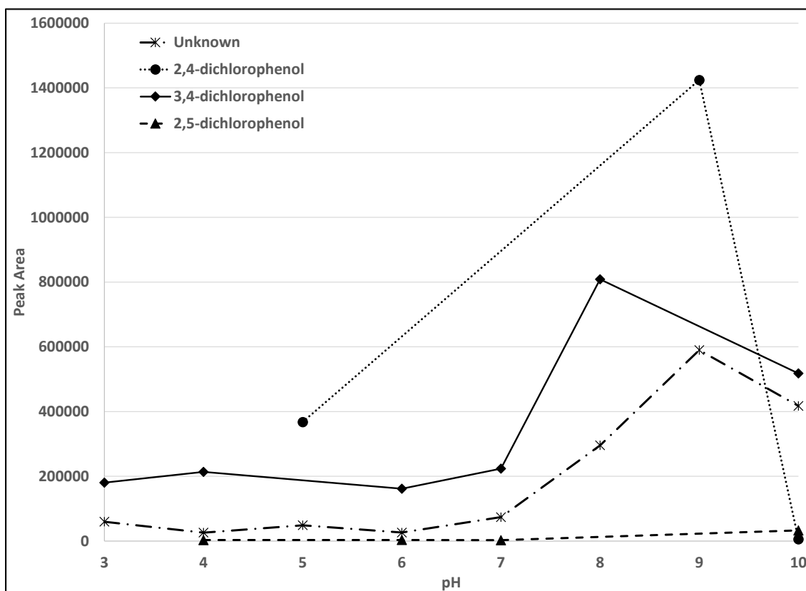
Figure 66. Comparison of the relative concentration (peak area) of 2,4-dichlorophenol, 2,5-dichlorophenol, 3,4-dichlorophenol, and the unknown based on reaction pH.
