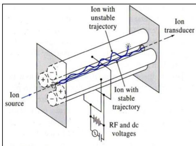
Figure 9. A single quadrupole mass analyzer 121 .
