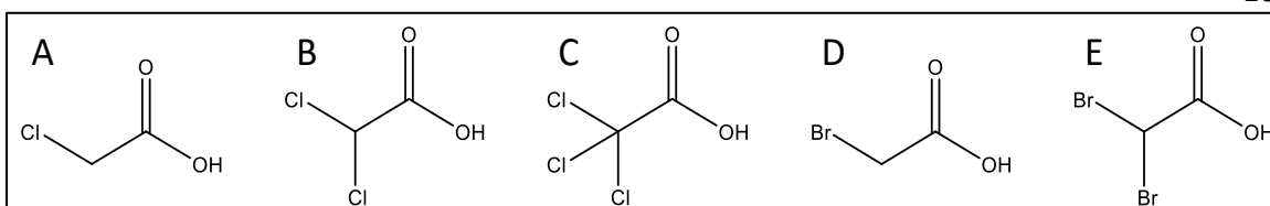
Figure 5. Structures of the five EPA regulated HAAs: (A) chloroacetic acid, (B) dichloroacetic acid, (C) trichloroacetic acid, (D) bromoacetic acid, and (E) dibromoacetic acid.
