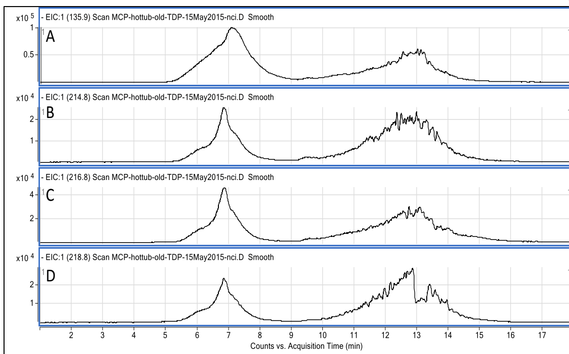
Figure 26. TD-NCI-TOF-MS extracted ion chromatograms for the (A) m/z 135.9 ion, (B) m/z 214.8 ion, (C) m/z 216.8 ion, and (D) m/z 218.8.
