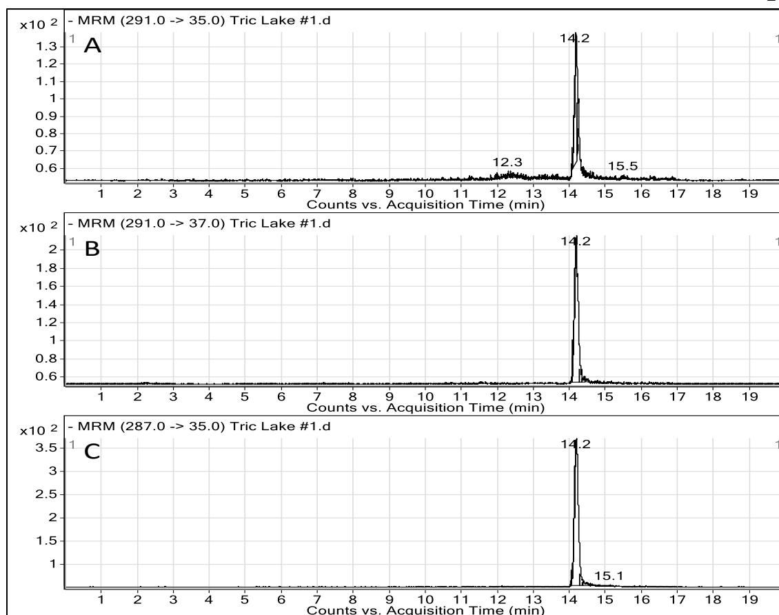
Figure 42. Extracted ion chromatograms indicating the presence of triclosan via the fragmentation of chlorine isotopes from selected isotopologues ((A) m/z 291 \rightarrow m/z 35, (B) m/z 291 \rightarrow m/z 37, and (C) m/z 287 \rightarrow m/z 35).
