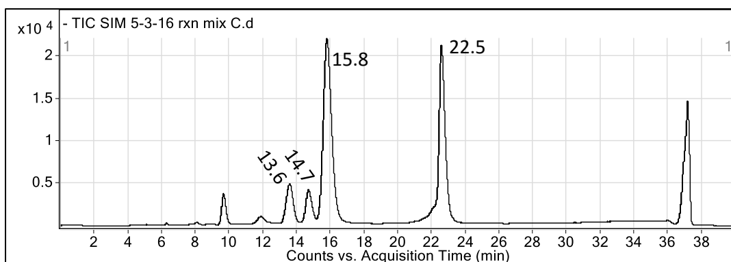
Figure 45. LC/MS/MS extracted ion chromatogram for m/z 161 from a reaction preformed at a pH of approximately 10.
