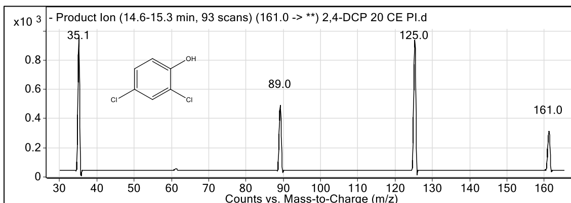
Figure 48. The structure of 2,4-dichlorophenol and its product ion spectrum of m/z 161 (the (M-H) - ion having a formula of ^{12}\text{C}_6\text{H}_3^{35}\text{Cl}_2\text{O} ).
