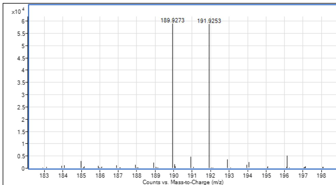
Figure 23. Mass spectrum of a monobrominated compound having monoisotopic masses at m/z 189.9273 and m/z 191.9253.
