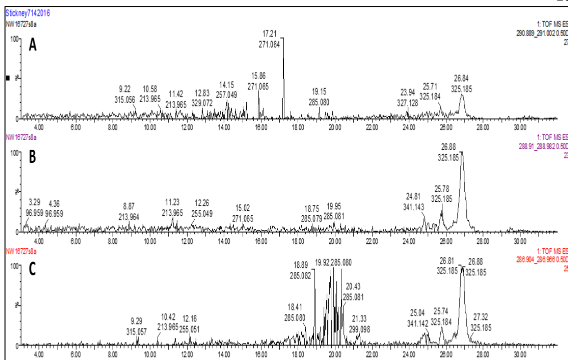
Figure 40. LC-TOFMS extracted ion chromatograms of the (A) m/z 290.9 ion, (B) m/z 288.9 ion, and (C) m/z 286.9 ion of the ^{35}\text{Cl} and ^{37}\text{Cl} isotopologues of triclosan.
