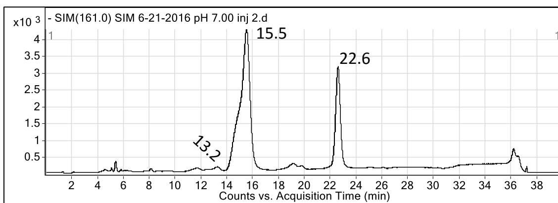
Figure 62. Extracted ion chromatogram of m/z 161 from a reaction performed at a pH of approximately 7.
